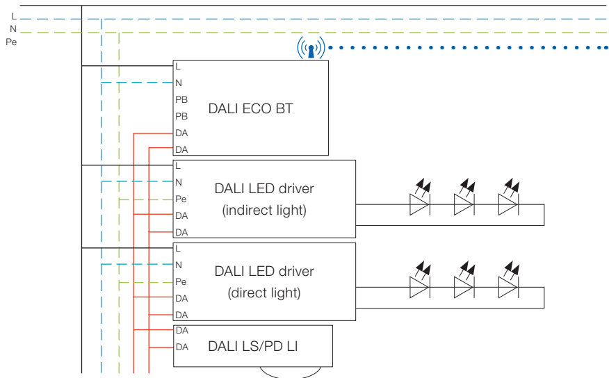
c) Wiring diagram of floor-standing luminaires shown in zones 1-4
